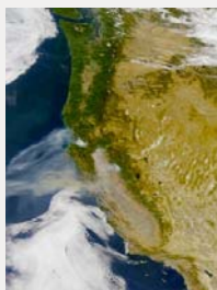
California Fires Visible Earth, NASA
